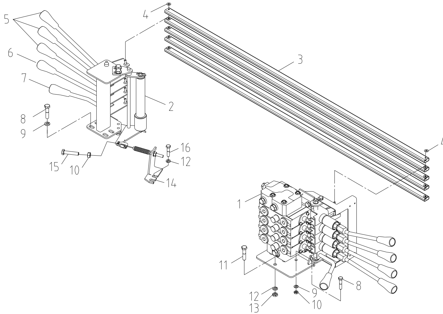
Fig. 3-3 SCS506 OPERATION MAIN ASS'Y
