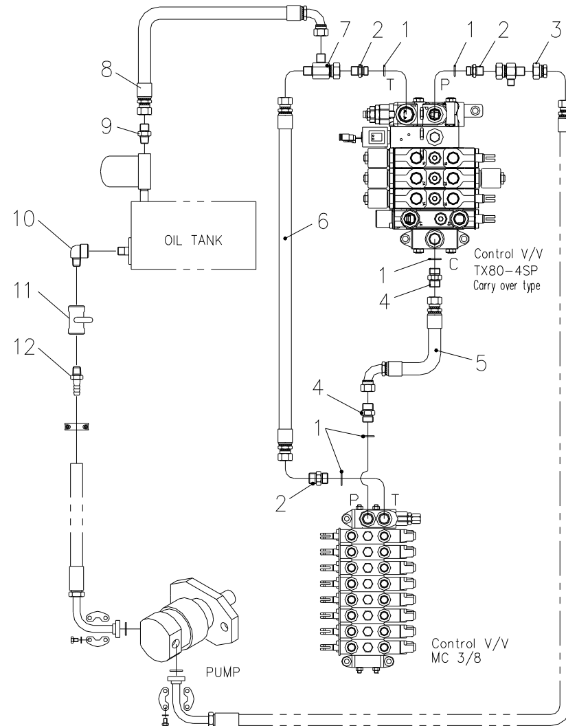
Fig. 5-1 SCS506 DISTRIBUTOR PIPING
