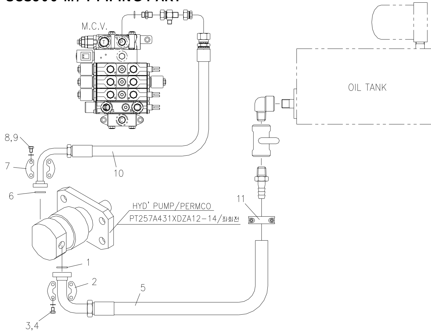
Fig. 8-3 SCS506 M/T PIPING PART
