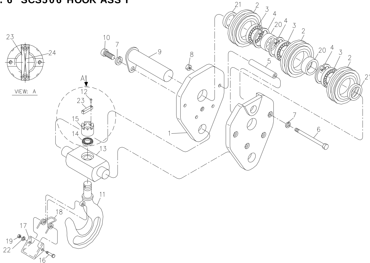
Fig. 6 SCS506 HOOK ASS'Y
