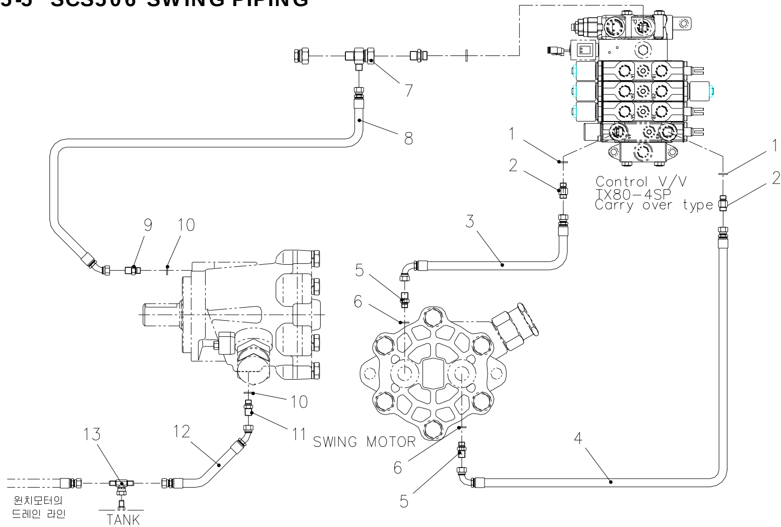
Fig. 5-5 SCS506 SWING PIPING
