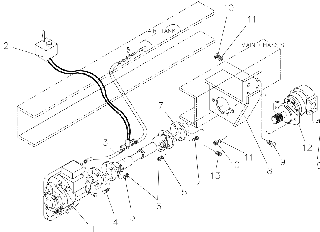
Fig. 8-1 SCS506 P.T.O &amp; PUMP PART ASS'Y
